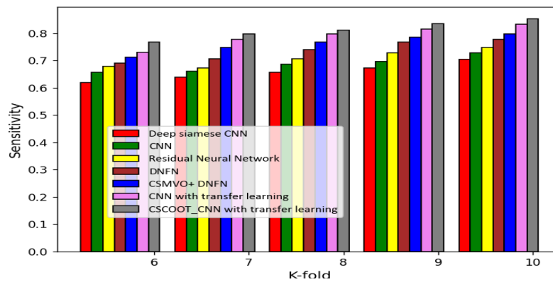
Fig.5(a). Evaluation based upon value of k-fold Sensitivity
